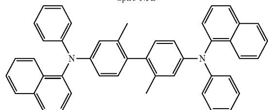
\alpha -NPB
