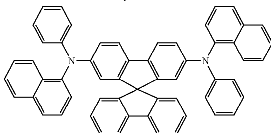
Spiro-NPB
