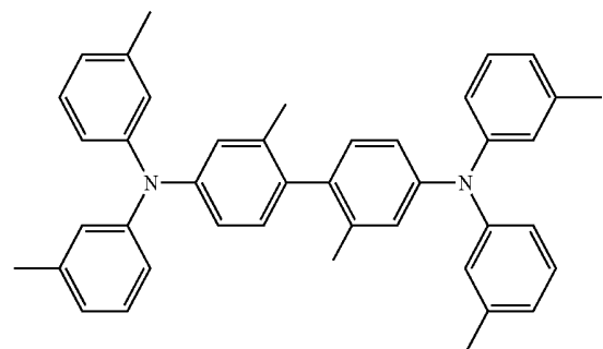
HMTDP
