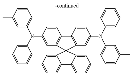
Spiro-TPD
